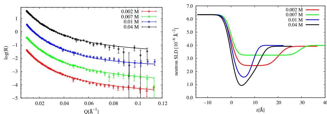
Figure 2: (Left) Data collected at the water/dodecane interface at various extractant concentrations in oil (shown in the legend). (Right) Corresponding SLD profiles obtained via best fit modelling.
