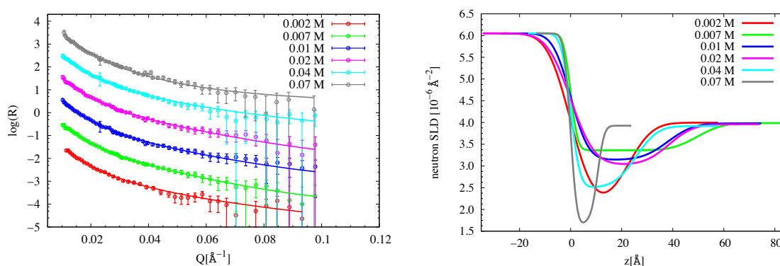
Figure 3: (Left) Data collected at the water/dodecane interface at various extractant concentrations in oil (shown in the legend). The aqueous phase was a Nitric acid aqueous solution (2 M). (Right) Corresponding SLD profiles obtained via best fit modelling.
