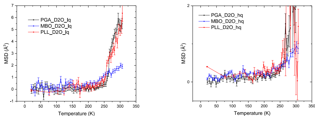
Figure 1 MSD values of the sample hydrated with D 2 O (empty cell subtraction was applied). Values were obtained from the \ln(I) vs Q^2 curves in the low momentum transfer range (left, 0.1 \text{ \AA}^{-2} < Q^2 < 3 \text{ \AA}^{-2} ) and the high momentum transfer range (right, 6.5 \text{ \AA}^{-2} < Q^2 < 15 \text{ \AA}^{-2} ).
