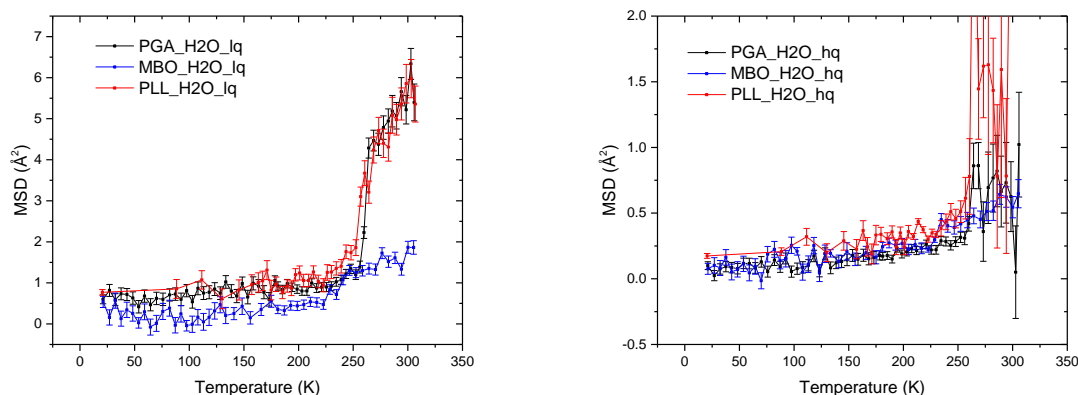
Figure 2 MSD values of the sample hydrated with H 2 O (empty cell subtraction was applied). Values were obtained from the \ln(I) vs Q^2 curves in the low momentum transfer range (left, 0.1 \text{ \AA}^{-2} < Q^2 < 3 \text{ \AA}^{-2} ) and the high momentum transfer range (right, 6.5 \text{ \AA}^{-2} < Q^2 < 15 \text{ \AA}^{-2} ).
