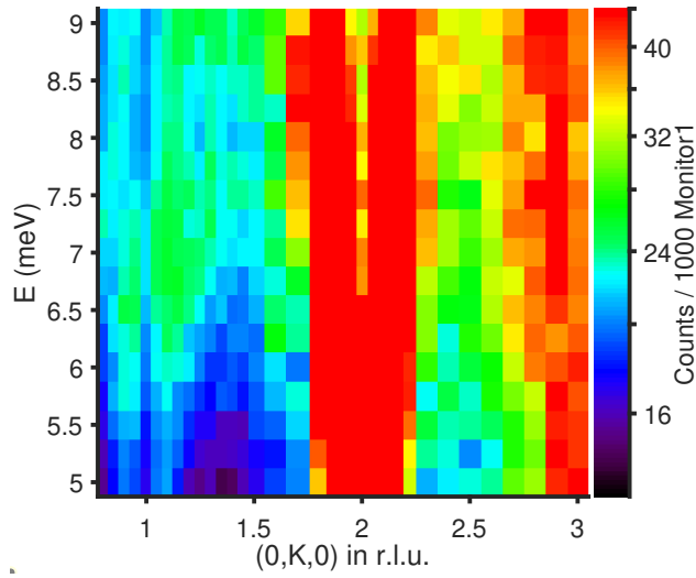
(c) Data from longitudinal measurements which show clearly the optical phonon modes as well as the weak novel excitation at about 6.5 meV to 7 meV.
