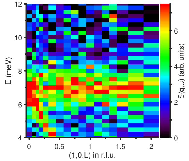
(b) Difference between 1.5 K data and 70 K scattering functions S(\mathbf{Q}, \hbar\omega) with Bose factor correction in the (1,0,L) - \hbar\omega plane.
