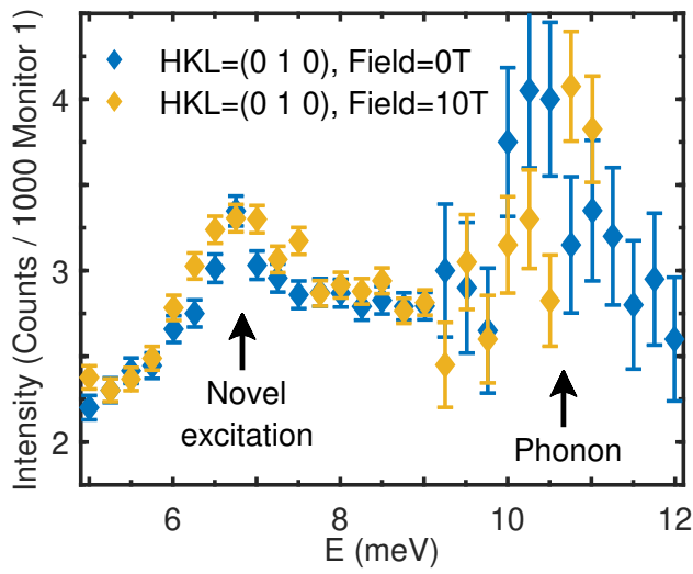
(a) The constant \mathbf{Q} -cut at (010) and 1.5 K shows significant broadening of the novel excitation at 10 T with respect to zero field which implies a shortened excitation's lifetime.
